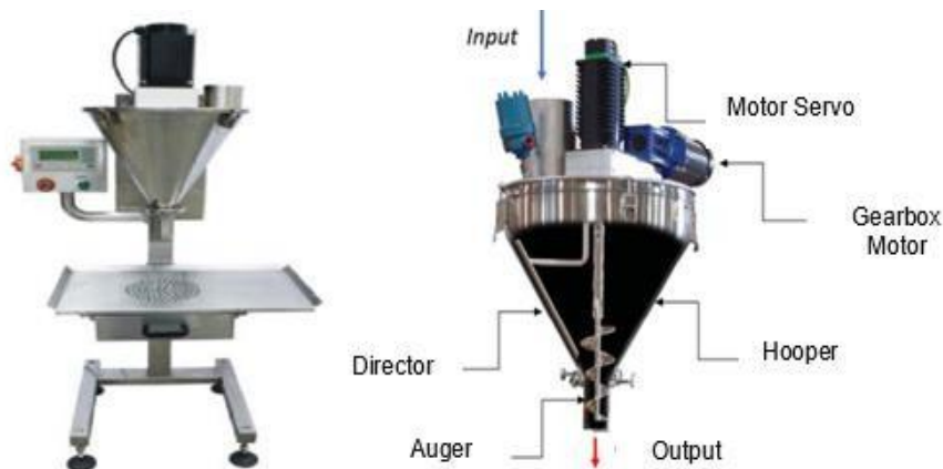
Figure 4. Fillmach S01P.
