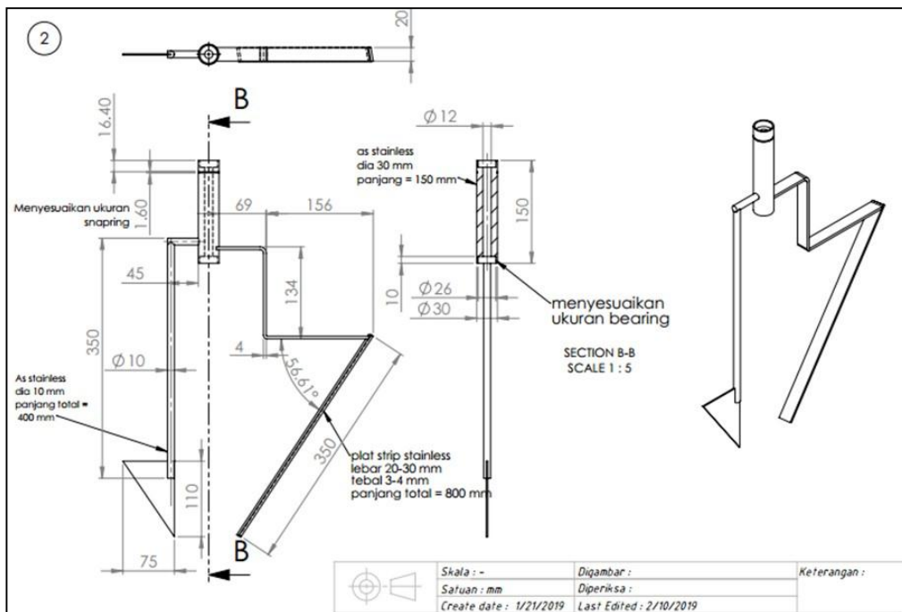
Figure 10. Redesign of Agitator.
