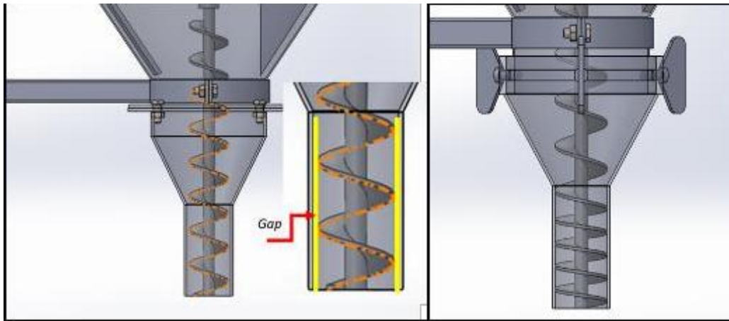
Figure 9. Redesign of Hooper.
