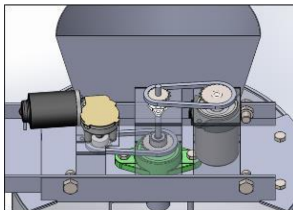
Figure 11. Redesign of transmission.
